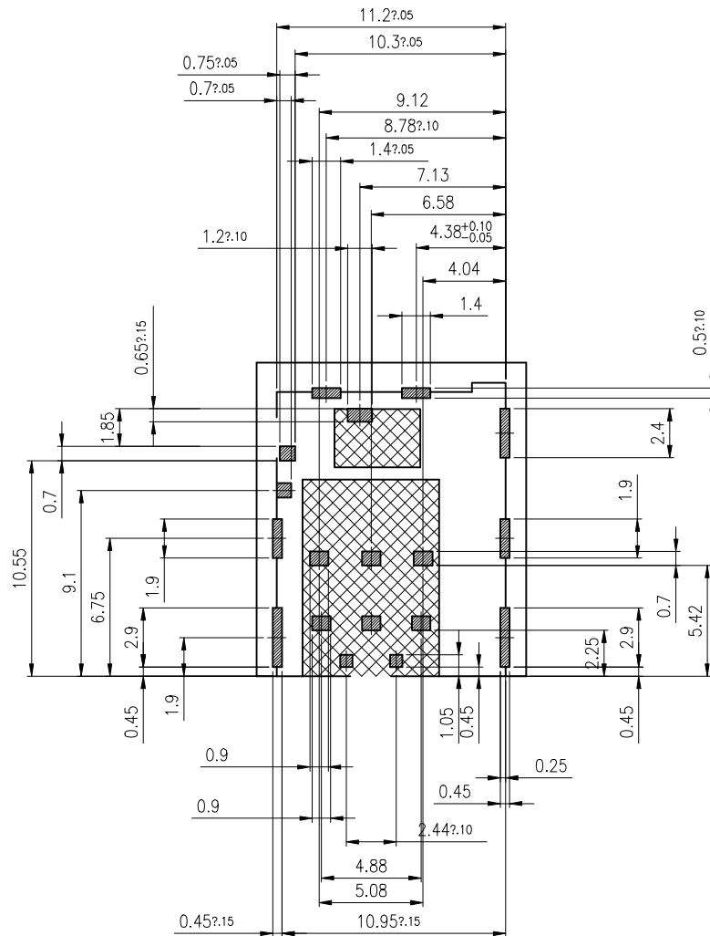
RECOMMENDED PCB LAYOUT TOP VIEW (TOLERANCE:±0.05) RECOMMENDED MATAL MASK T=0.12MM
