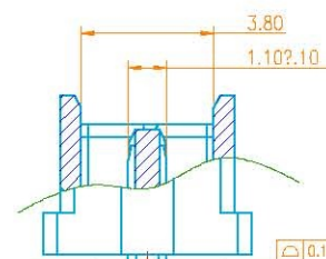
SECTION: A-A SCALE 2:1
